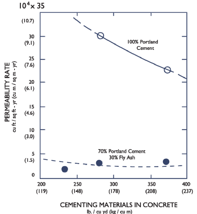
Permeability of concrete with and without pozzolan. Elfert, R.J. "Bureau of Reclamation Experiences with Fly Ash and Other Pozzolans in Concrete", Third International Ash Utilization Symposium, 1973, p. 14.
