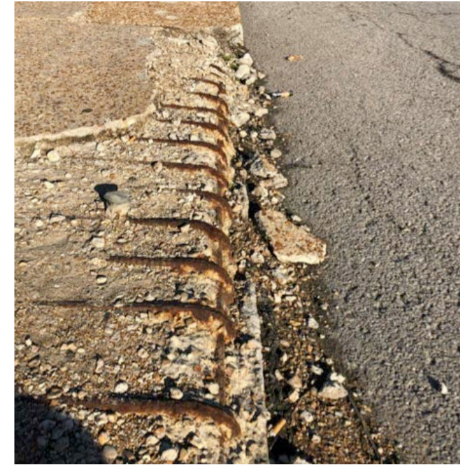
FIGURE 2: CONCRETE CRACKING AND DELAMINATION CAUSED BY CORROSION OF STEEL REINFORCEMENT
