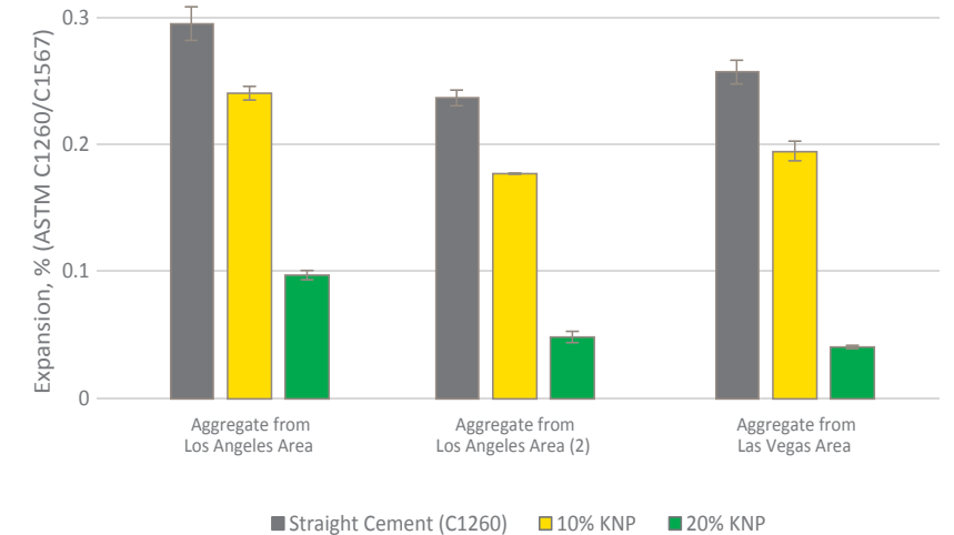
FIGURE 4: EXPANSION CAUSED BY ASR MEASURED ACCORDING TO ASTM C1567 USING AGGREGATES FROM THE LOS ANGELES AND LAS VEGAS AREAS AND PROPORTIONED WITH INCREASING AMOUNTS OF KNP
