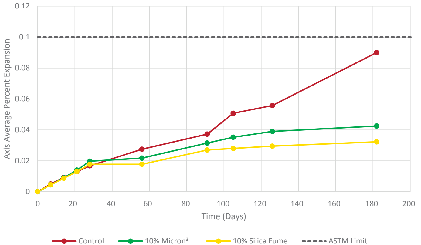
FIGURE 12: ASTM C1012 RESULTS
