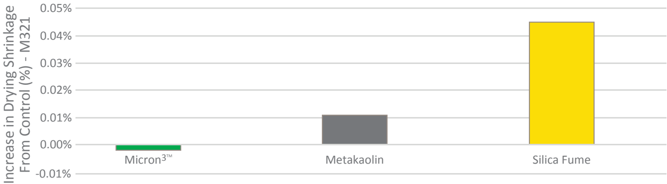
FIGURE 7: DRYING SHRINKAGE PER AASHTO M321
