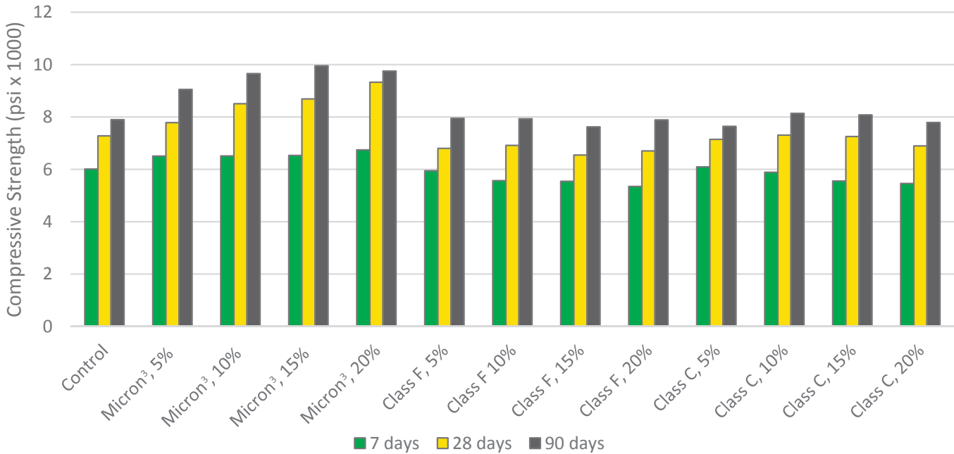
FIGURE 4: STRENGTH DEVELOPMENT
